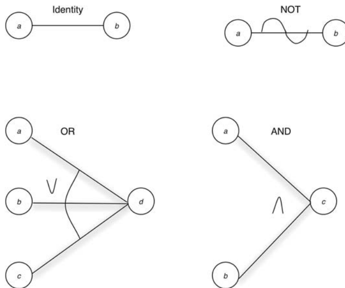
FIGURE 4.5 Basic Cause-Effect Graph Symbols.
