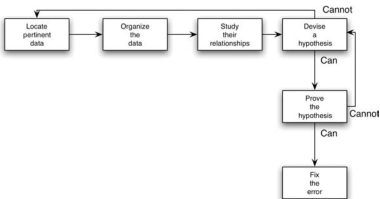
FIGURE 8.1 The debugging process.
