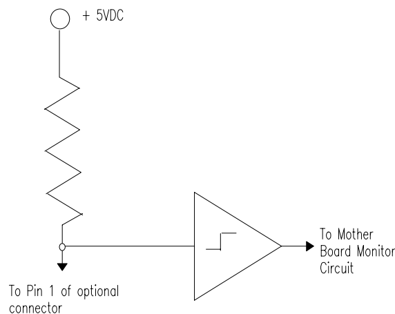
Figure 11: Simple Implementation of a Fan Monitor Circuit
