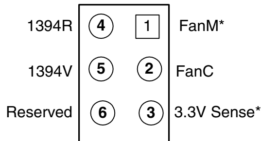
Figure 10: 6-pin Optional Power Supply Connector Configuration
