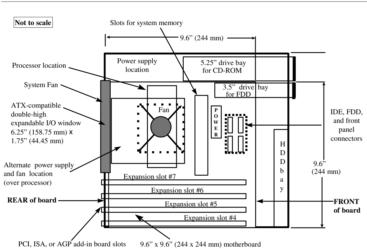
Figure 1: Example of a microATX System
