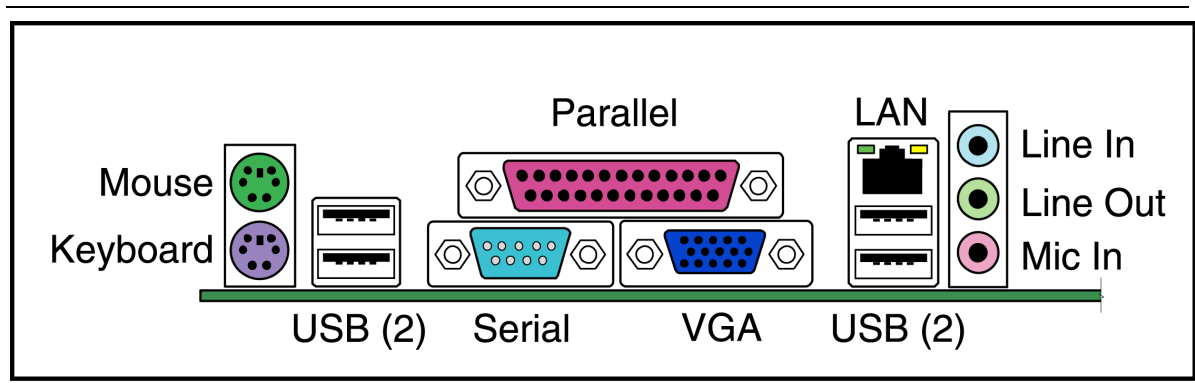
Figure 6: Example Rear Panel I/O Connector Layout
