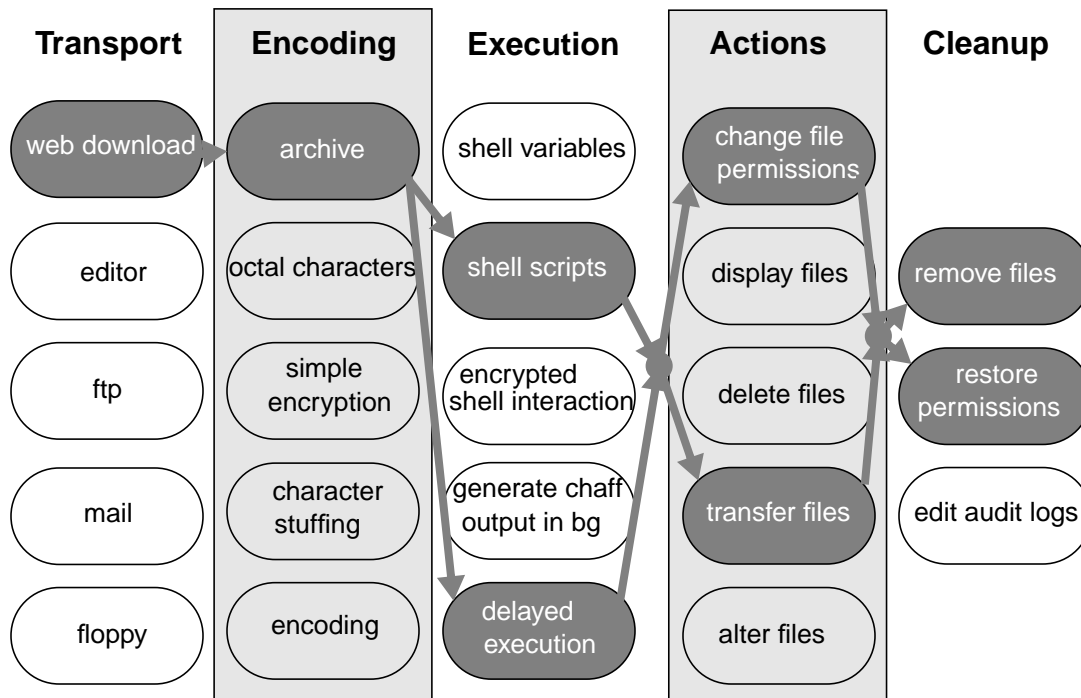
Figure 5.7: Path of a ps Attack
